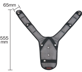
KPCKRD-YBF
